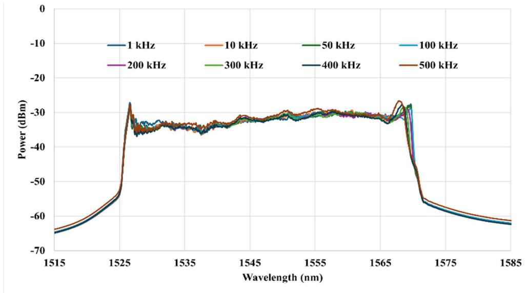
Figure 1. 1550nm Swept Laser Source at different scan speeds.
